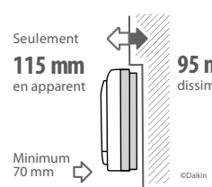
Pose semi-encastree
